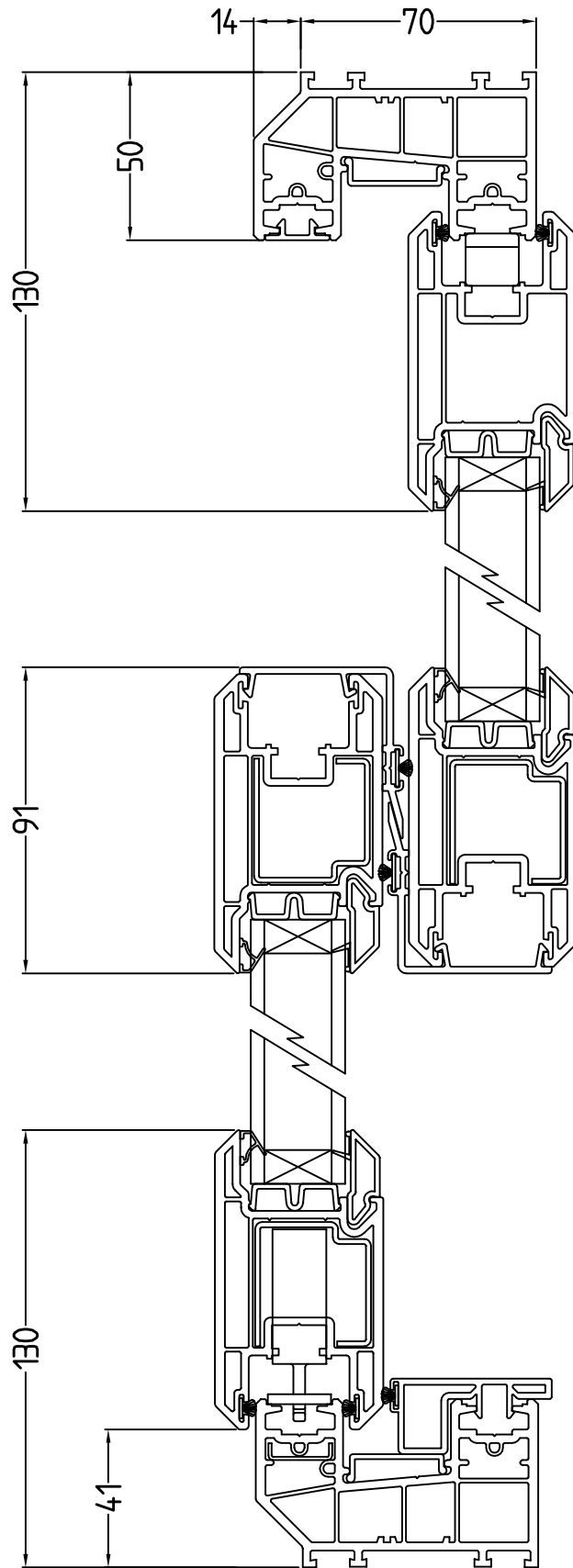
HORIZONTAL CROSS SECTION (2 PANE STYLE)
