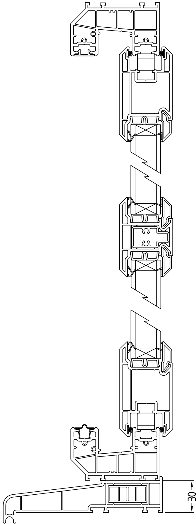
TYPICAL VERTICAL SECTION THROUGH FIXED SASH.
