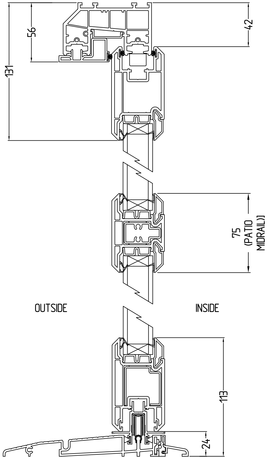
TYPICAL VERTICAL SECTION THROUGH SLIDING SASH.
