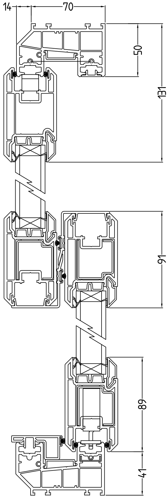
HORIZONTAL CROSS SECTION (2 PANE STYLE)
