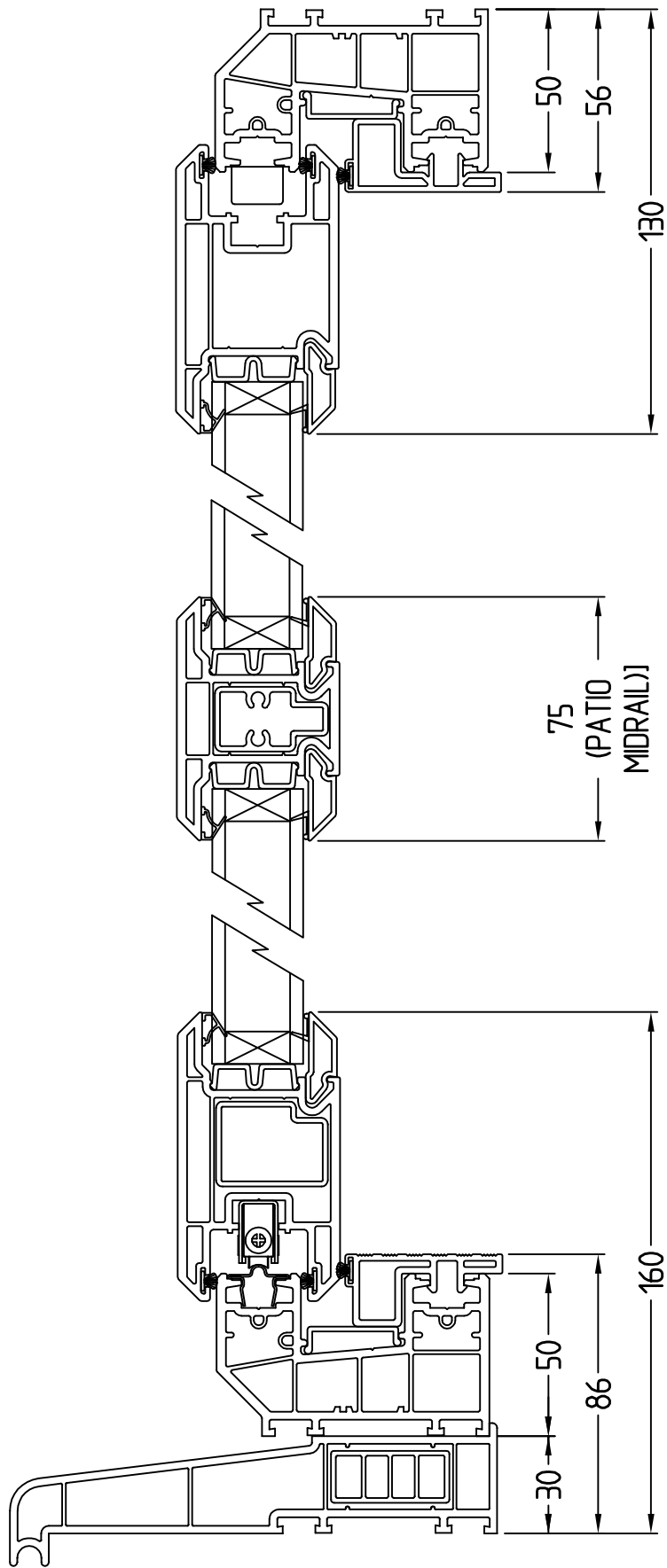
TYPICAL VERTICAL SECTION THROUGH SLIDING SASH.
